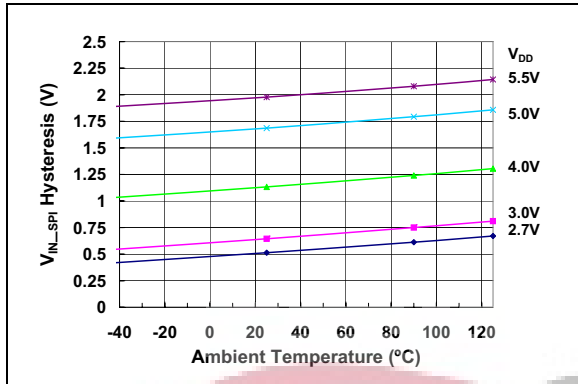
FIGURE 2-23: V_{m\_spl} Hysteresis vs. Ambient Temperature and V_{DD} .
